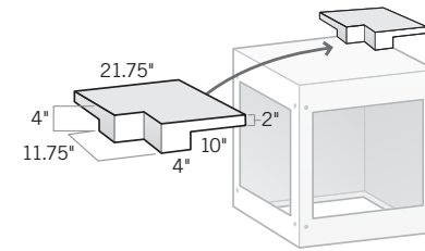
Corner Raised Backsplash OLPLSBCRN Creates 4" high raised corner backsplash with 10" cantilever; connects to Straight Raised Backsplash for L-shaped configurations. Requires 2 bolts for mounting (not included).
