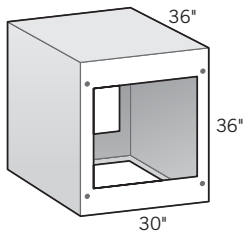
36" Cabinet 30"D × 36"H • OLPLS0036
