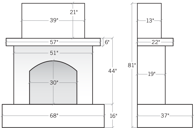
Gas-Burning Fireplace 37"D × 68"L × 81"H • OLPLSFP01
