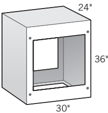
24" Cabinet 30"D × 36"H • OLPLS0024
