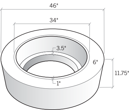
Fire Pit 46" DIAMETER x 11.75" H • 0LPLSFP48
